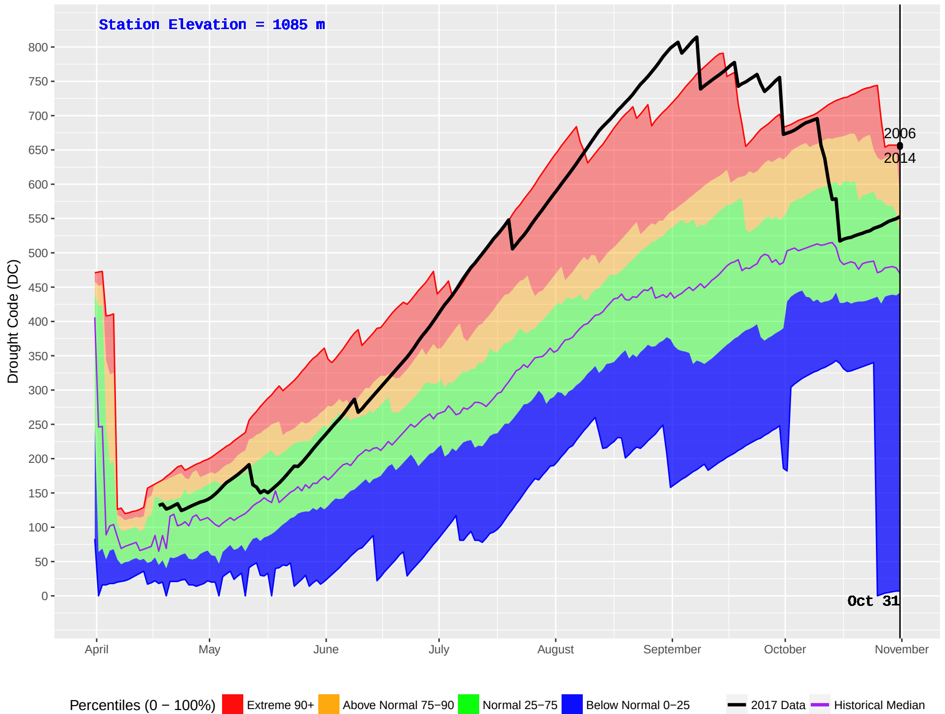
TAUTRI (206) : Historical (1970–2016) and Current (2017) Noon Drought Code (DC)
