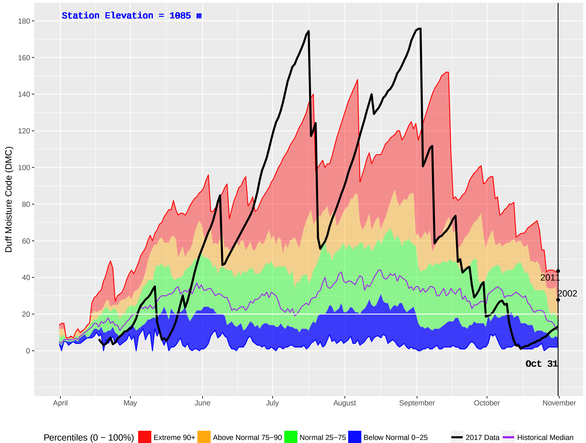
TAUTRI (206) : Historical (1970–2016) and Current (2017) Noon Duff Moisture Code (DMC)
