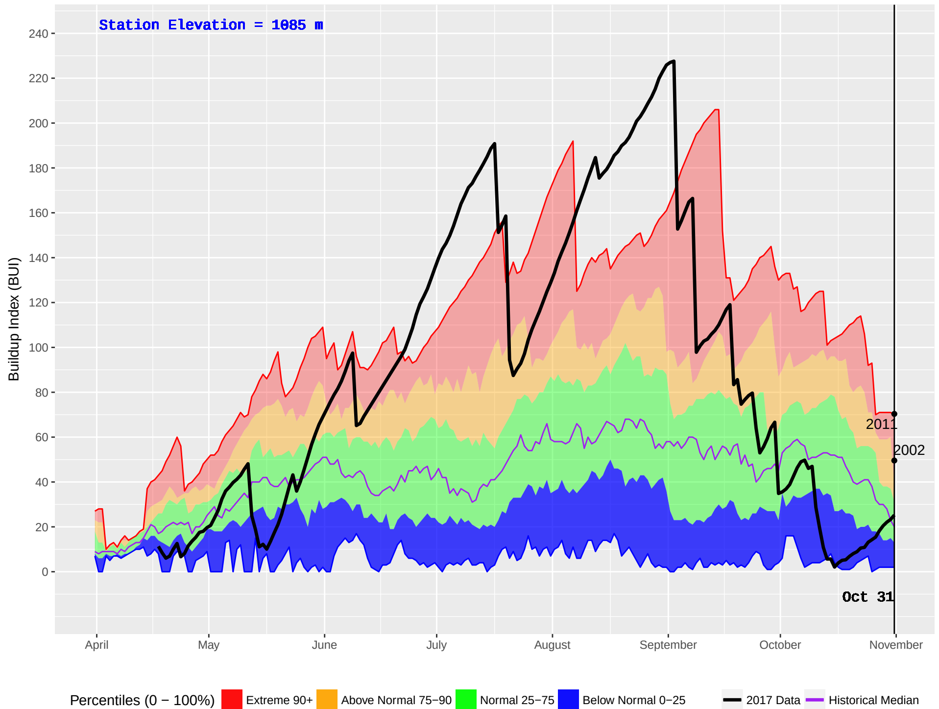
TAUTRI (206) : Historical (1970–2016) and Current (2017) Noon Buildup Index (BUI)
