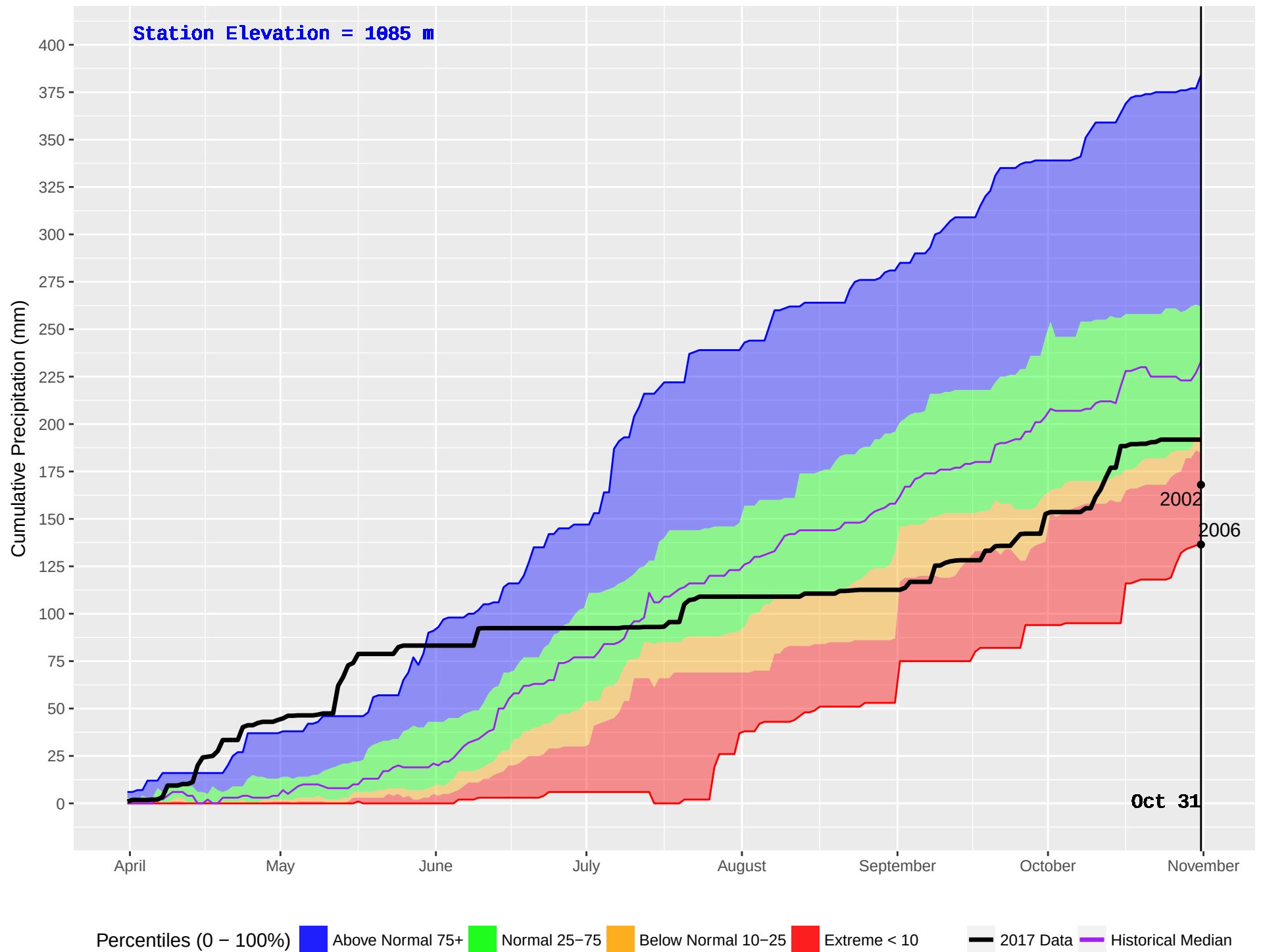
TAUTRI (206) : Historical (1970–2016) and Current (2017) Noon Cumulative Precipitation
