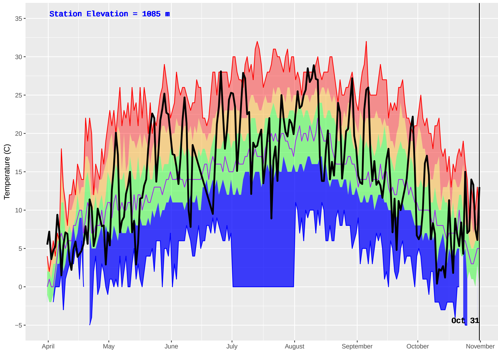
TAUTRI (206) : Historical (1970–2016) and Current (2017) Noon Temperature
