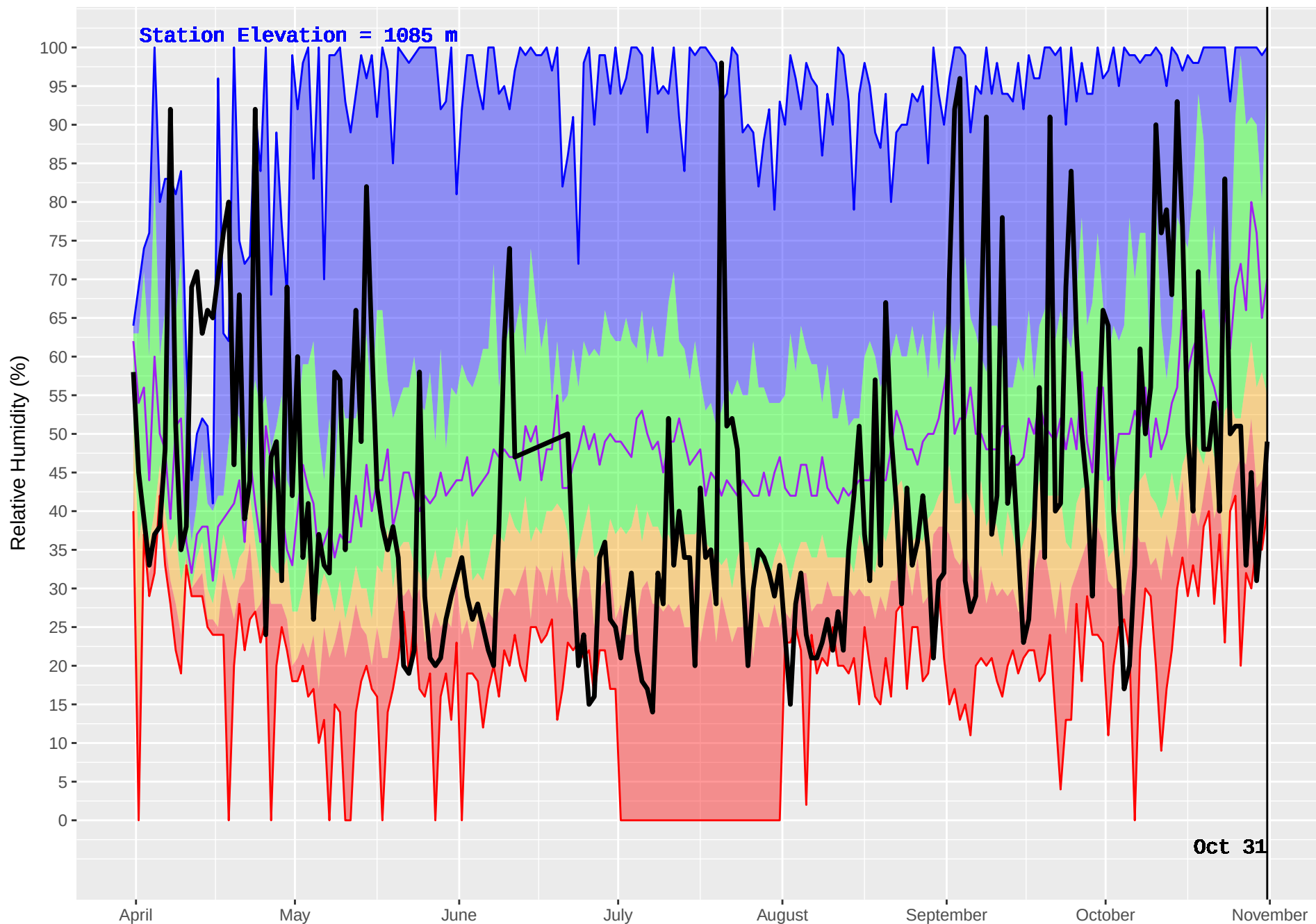
TAUTRI (206) : Historical (1970–2016) and Current (2017) Noon Relative Humidity
