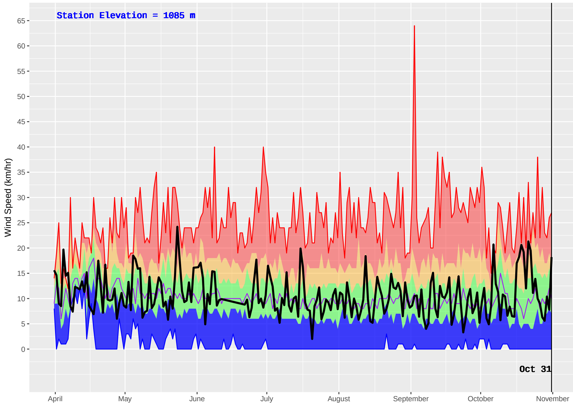
TAUTRI (206) : Historical (1970–2016) and Current (2017) Noon Wind Speed
